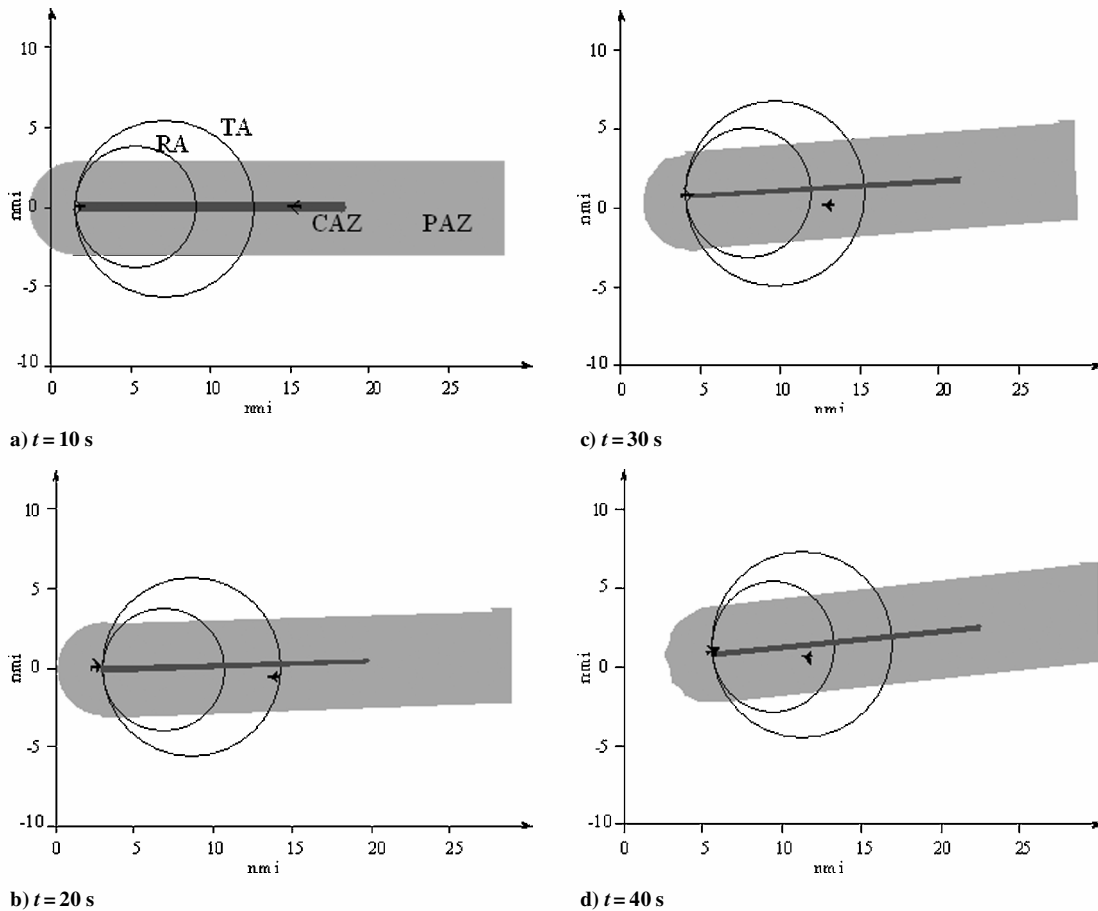
Fig. 6 TCAS and ACM thresholds during avoidance maneuver.
