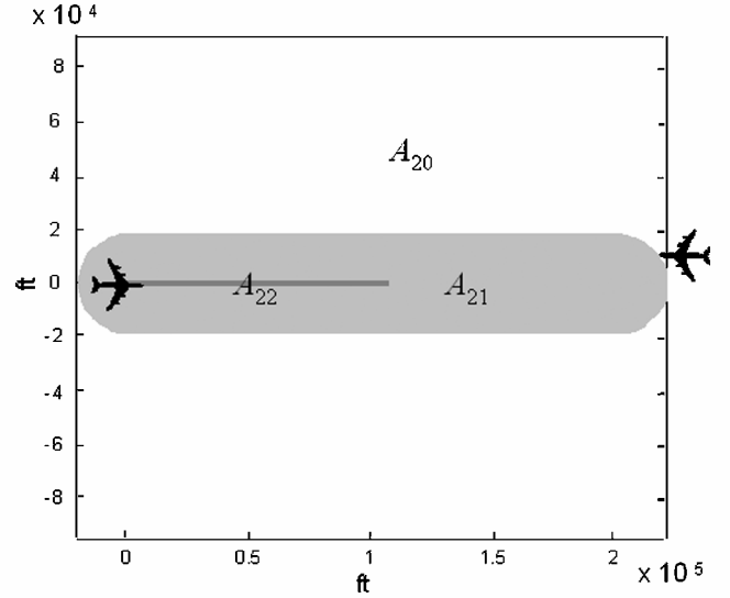
Fig. 3 Example ACM threshold function and alert stages, opposite direction aircraft at 500 kn each: A_{21} = PAZ alert and A_{22} = CAZ alert.
