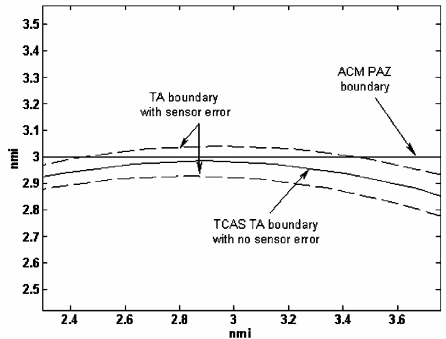
Fig. 5 Closeup of the effect of sensor error on TCAS TA boundary, 260 kn opposite direction.
