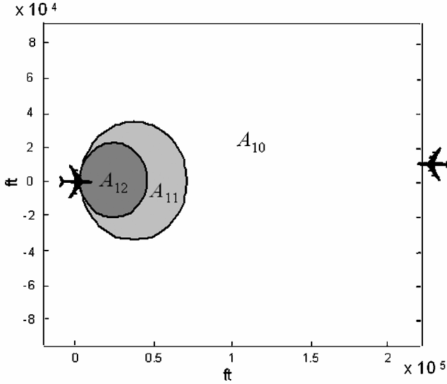
Fig. 2 Example TCAS threshold function and alert stages, opposite direction aircraft at 500 kn each: A_{10} = no alert, A_{11} = TA, and A_{12} = RA.
