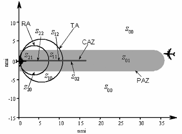
Fig. 4 Example TCAS and ACM thresholds, opposite direction aircraft at 500 kn each.
