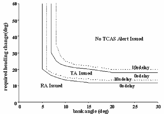
Fig. 7 Effect of PAZ avoidance maneuver on TCAS alert status, 500 kn opposite direction.
