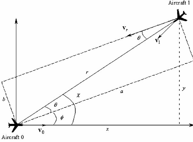
Fig. 1 Horizontal plane kinematics.
