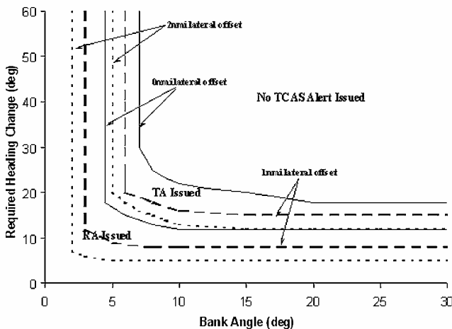
Fig. 9 Effect of lateral offset on PAZ avoidance maneuver for TCAS alert status, 500 kn opposite direction.
