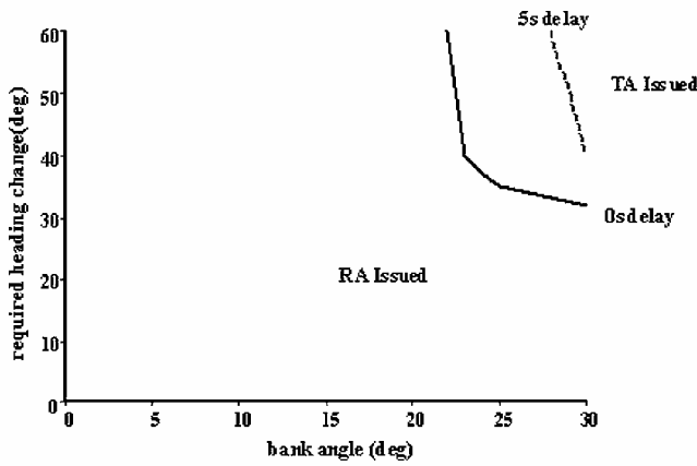
Fig. 8 Effect of CAZ avoidance maneuver on TCAS alert status, 500 kn opposite direction.
